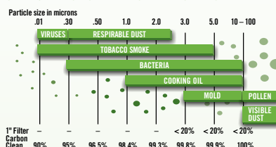
PARTICLE-REMOVAL EFFICIENCY — HEALTHY CLIMATE AIR CLEANERS
